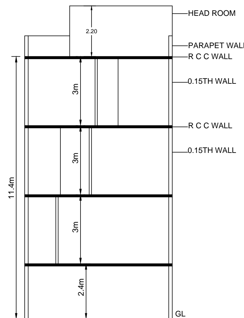
SECTION@X-X
